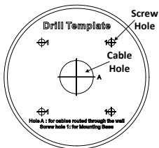
Figure 2-12 Drill Template of the Junction Box
