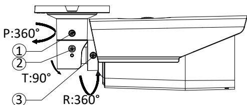
Figure 2-3 3-axis Adjustment
