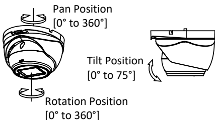
Figure 2-11 3-axis Adjustment
