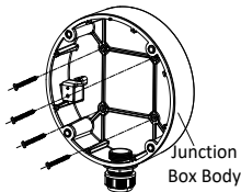
Figure 2-14 Secure the Junction Box's Body on Ceiling
