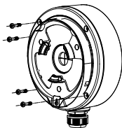
Figure 2-15 Fix the Junction Box
