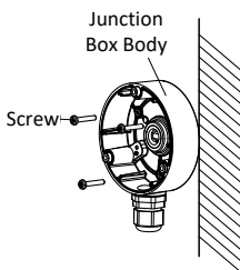
Figure 2-5 Fix the Camera to the Ceiling
