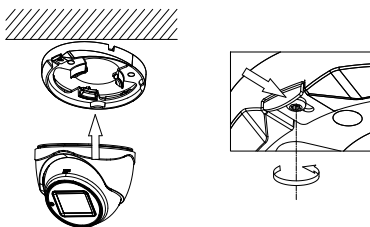
Figure 2-10 Install the Turret Camera
